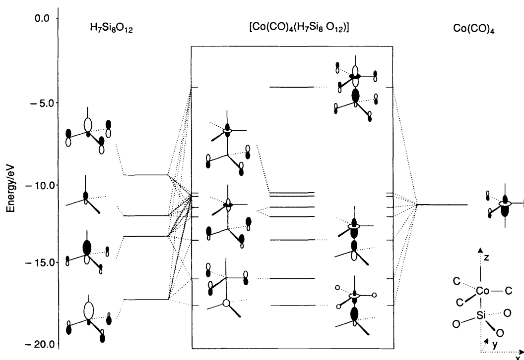
Fig. 7 Region B molecular orbitals of [\text{Co}(\text{CO})_4(\text{H}_7\text{Si}_8\text{O}_{12})] which are correlated in Fig. 6 to the orbitals of the two fragments
