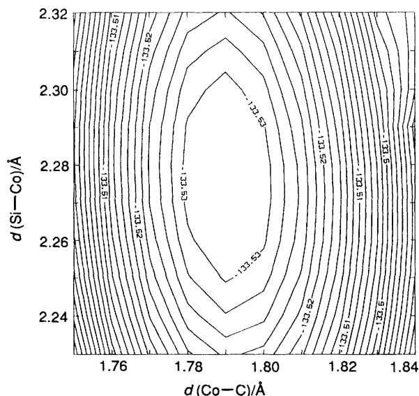
Fig. 4 Potential energy surface E_{(tot)} of [Co(CO) 4 (H 7 Si 8 O 12 )] for the Si–Co and the Co–C stretching motion
