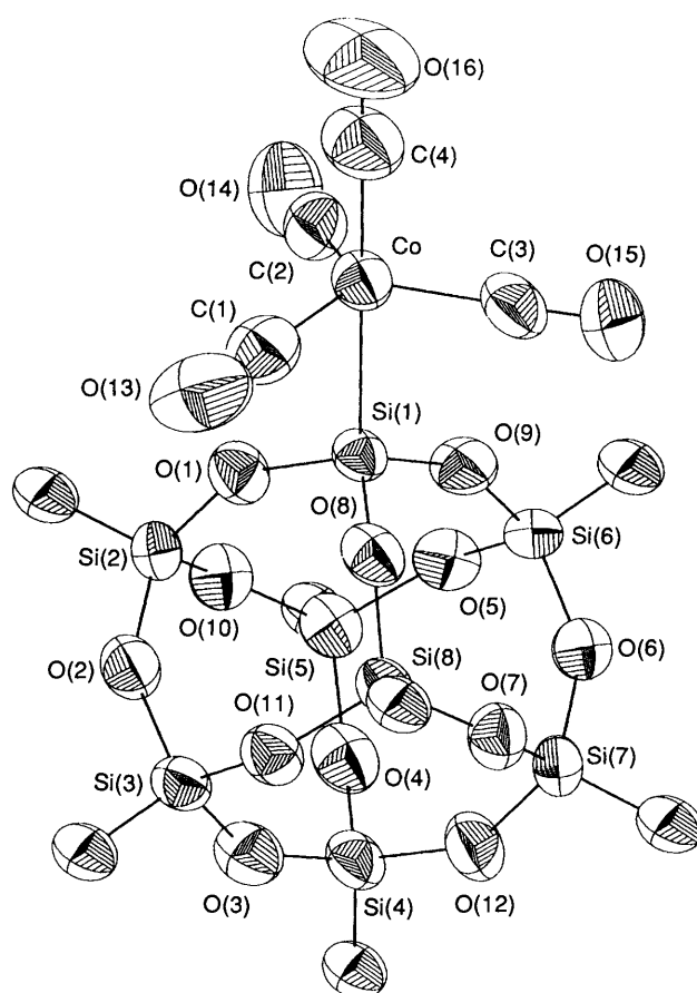
Fig. 2 The crystal structure of [\text{Co}(\text{CO})_4(\text{H}_7\text{Si}_8\text{O}_{12})] , displayed with atomic labelling and anisotropic thermal parameters at the 50% probability level
