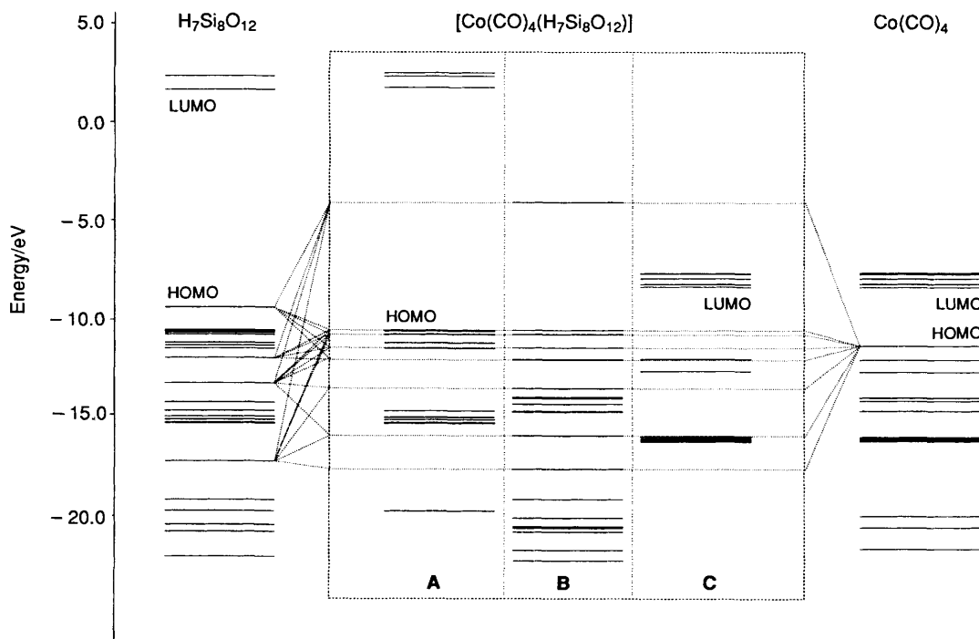
Fig. 6 Correlation diagram for H 7 Si 8 O 12 + Co(CO) 4 → [Co(CO) 4 (H 7 Si 8 O 12 )]. The energy levels of [Co(CO) 4 (H 7 Si 8 O 12 )] are split into three parts. Parts A and C contain the orbitals localised on the H 7 Si 8 O 12 and on the Co(CO) 4 fragment, respectively. The molecular orbitals of region B are delocalised over the whole molecule
