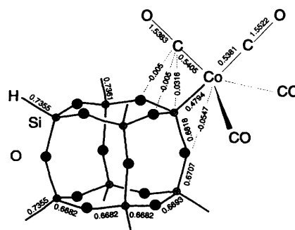
Fig. 5 Overlap population of [Co(CO) 4 (H 7 Si 8 O 12 )]
